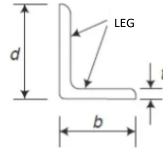
ANGLE (UNEQUAL)
