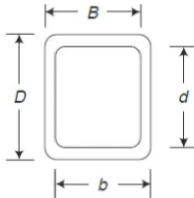
RECTANGULAR HOLLOW SECTION (HSS)
