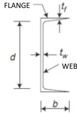
CHANNEL
